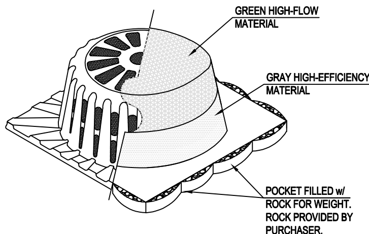
ISOMETRIC ASSEMBLY VIEW OF S200A-DOT
